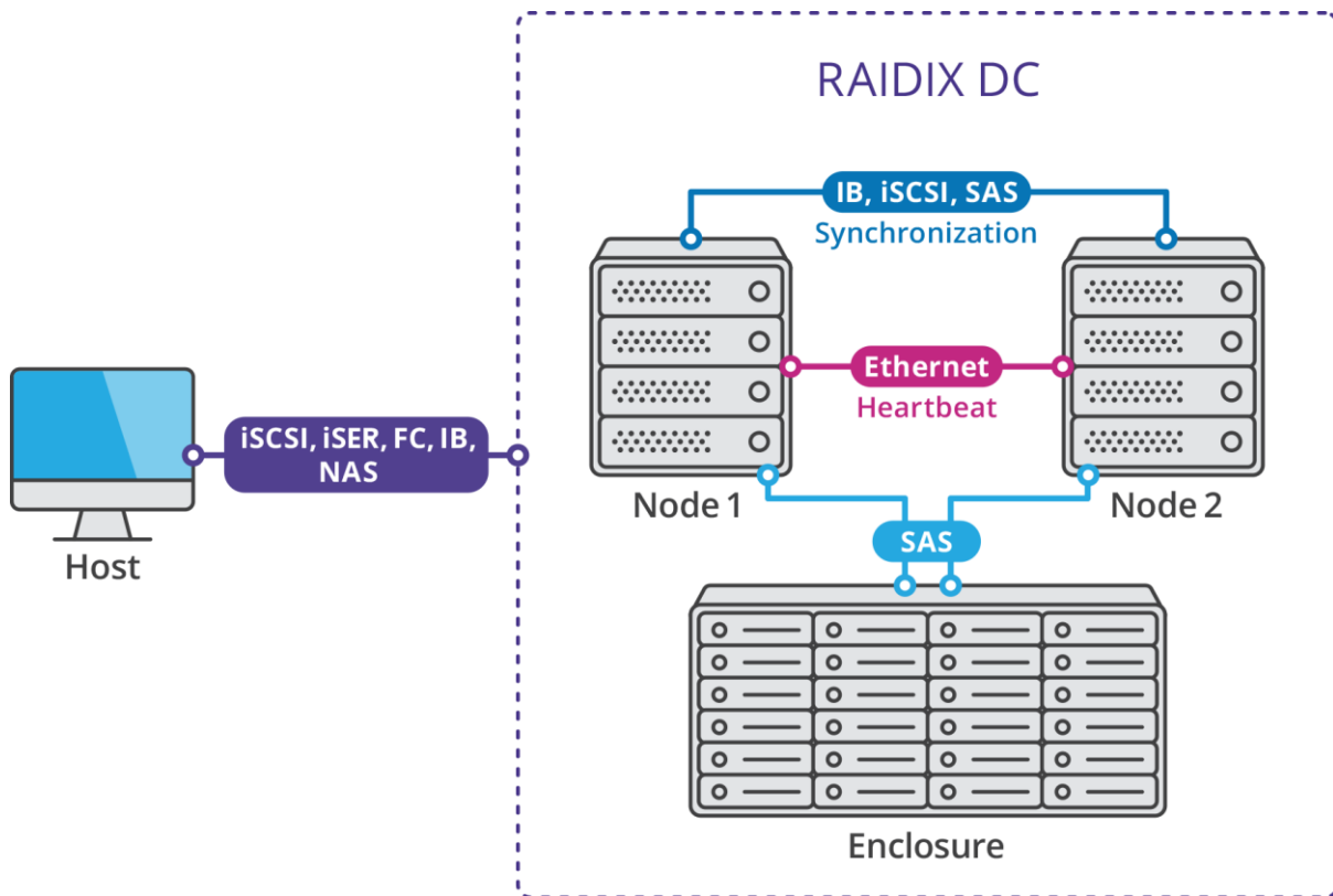
Figure 2. RAIDIX 5.2 Dual-controller mode
